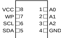
(MLP 2x3) Bottom View
